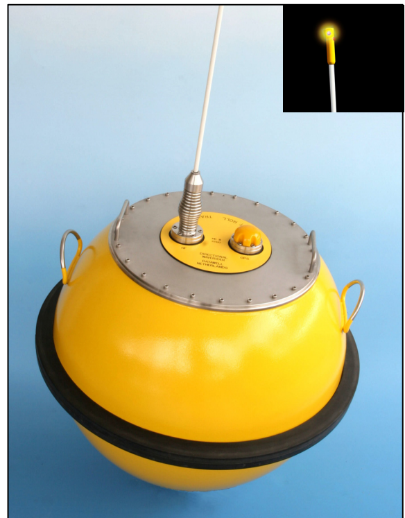
0.7 m (Hull painting is optional, not standard)
